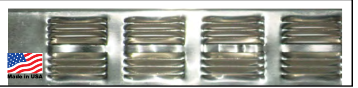
16" x 8" UNDEREAVE VENTS Aluminum construction · 8 mesh aluminum screen · NFA: 56 sq. in. per vent 24 Pieces/Carton · 60 Cartons/Pallet EV16824MF/84210 EV16824WH/84211 EV16624BR/84212 MILL FINISH WHITE BROWN
