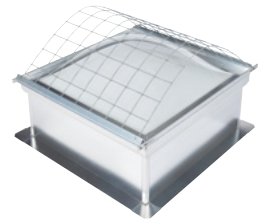
CAEW/CAEB/CAES Exterior Safety Screens (5" o.c. both directions)
